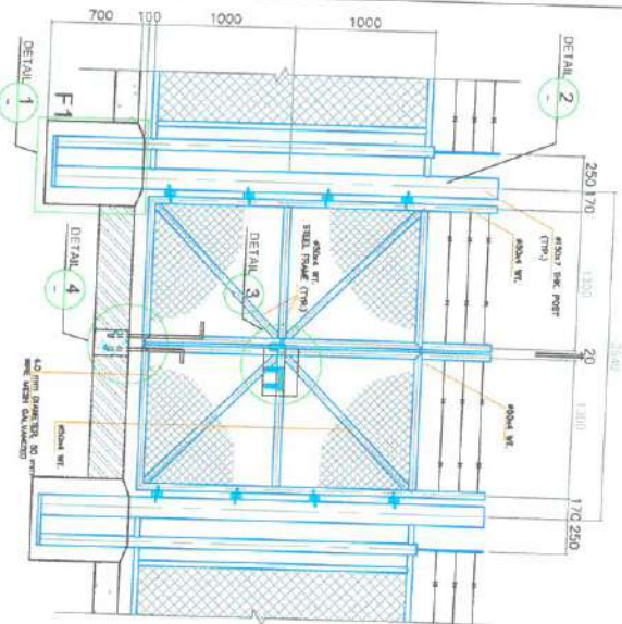
ELEVATION-TYPICAL DETAIL OF METALLIC STRETCHER
