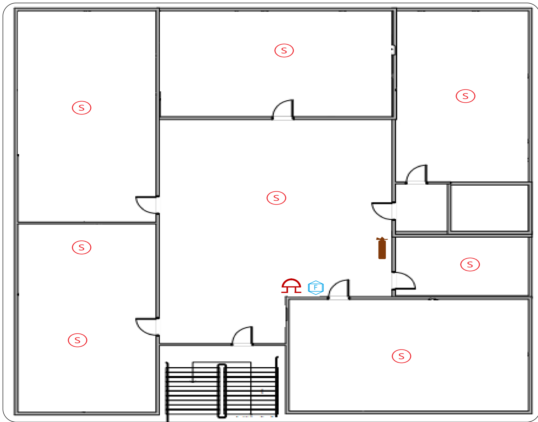
Fire alarm Plan of first floor
