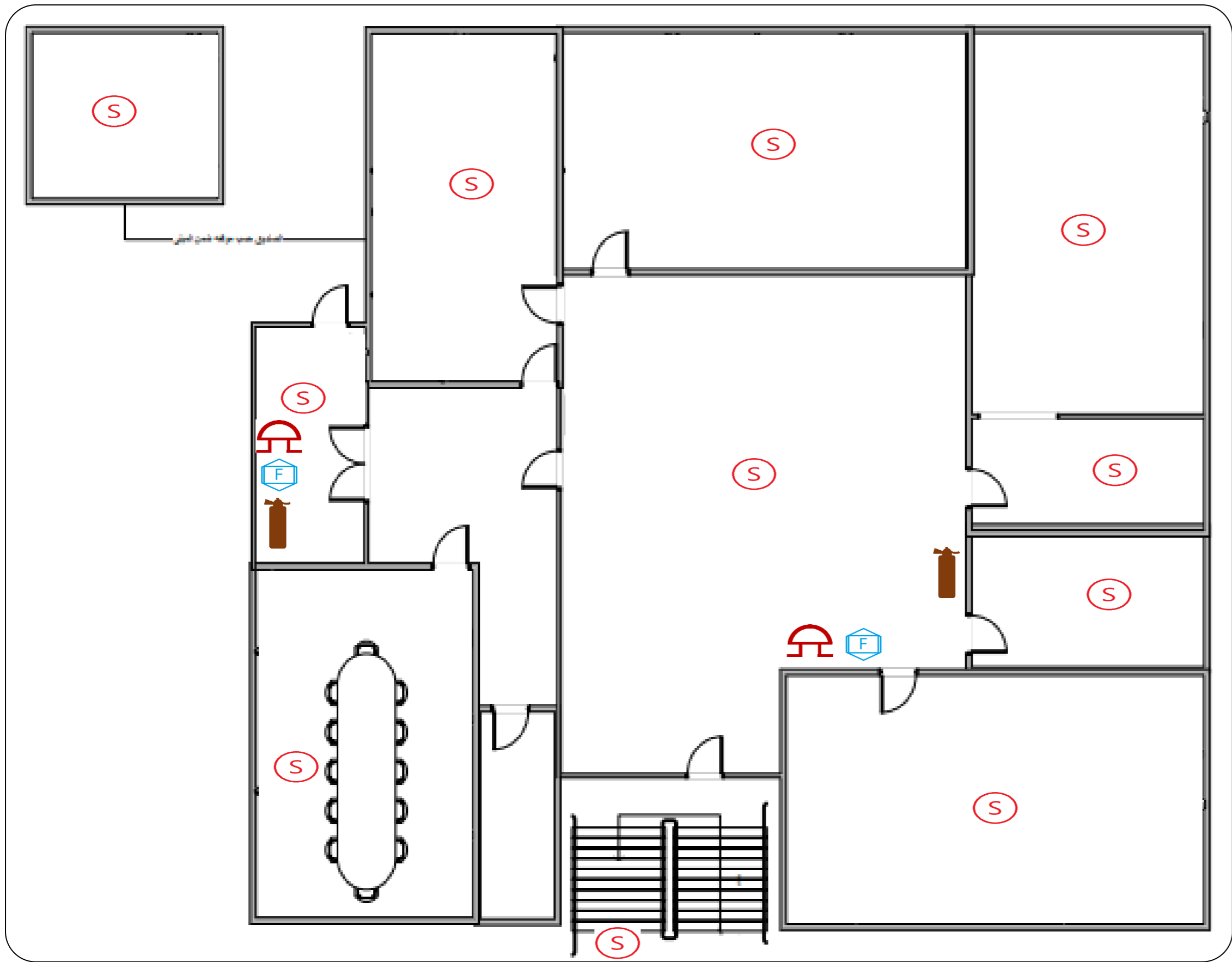
Fire alarm Plan of ground floor
