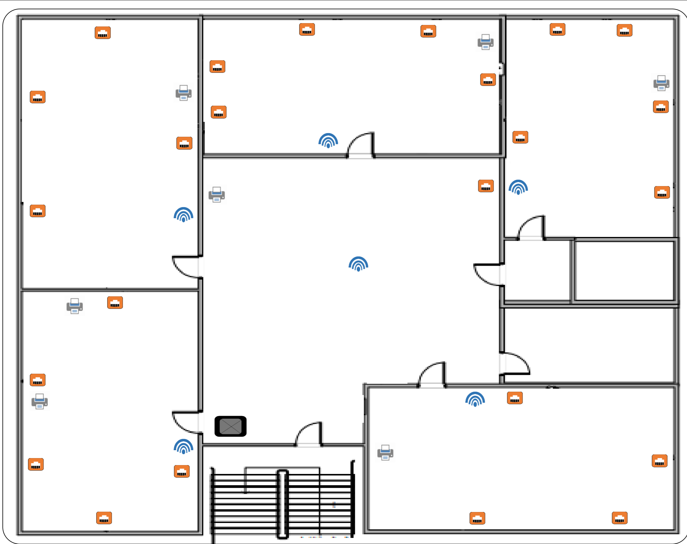
Network Plan of first floor
