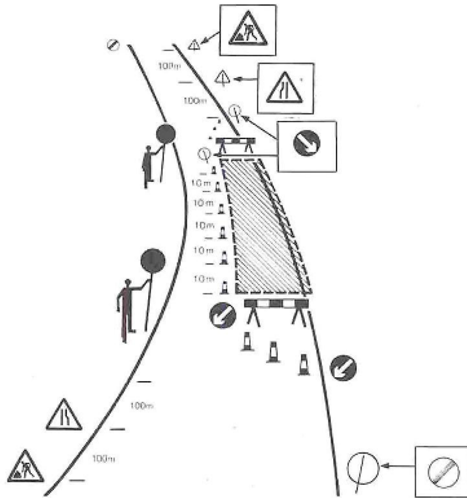
Figure 101 Sign layout for lane closure
