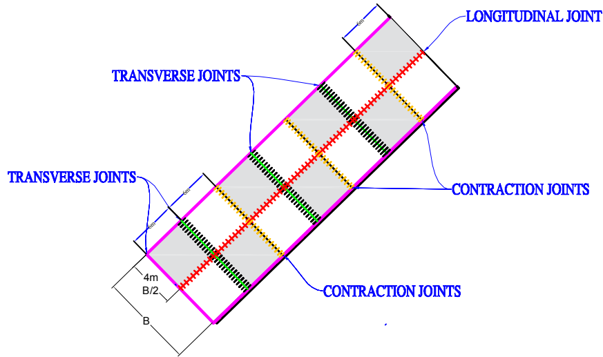
1 PLATFORM RIGID PAVEMENT PLAN STRUCTURE DETAILS
