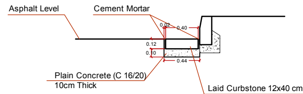
Laid Curbstone Typical
