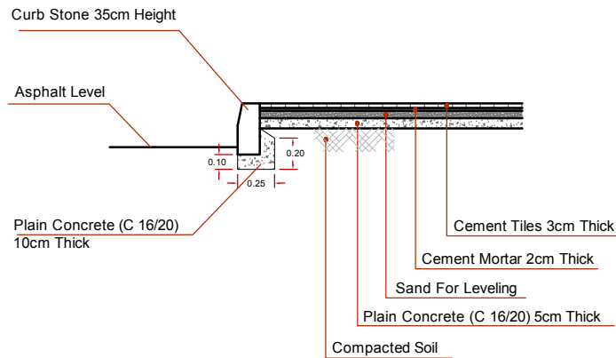
Detail 01
